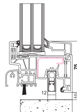
O60x27 + AMS 1227A
