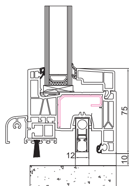
160x20 + AMS 1227A
