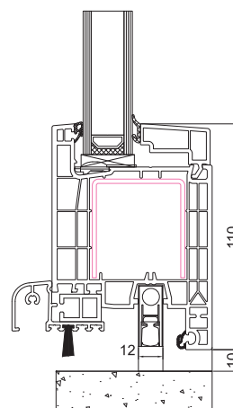
160x30 + AMS 1227A
