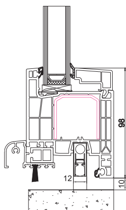
160x22 + AMS 1227A
